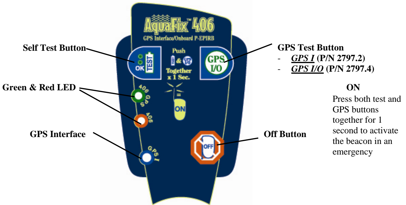
Figure 1. Key Pad Functions (P/N 2797.4 shown)
