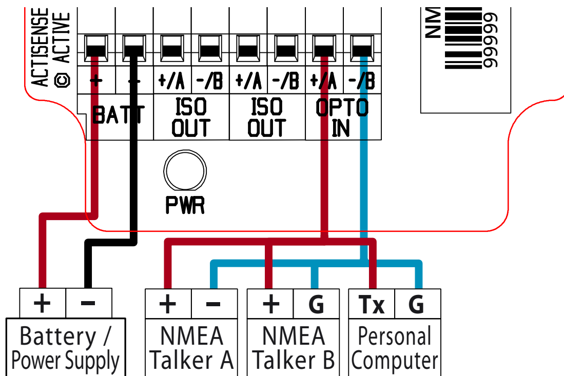
Figure 2 – Input connections
