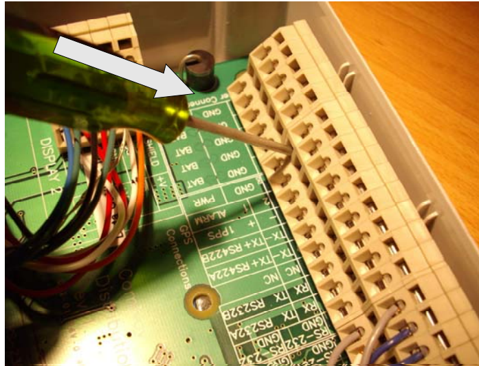
Figure 6 - Terminal Connection - Step 1
