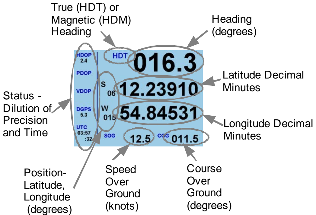
Figure 17 - Position Navigation Page Description
