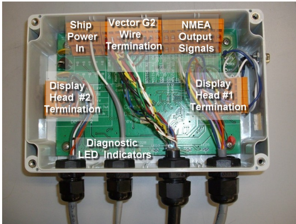
Figure 5 – Distribution Unit Connector Blocks
