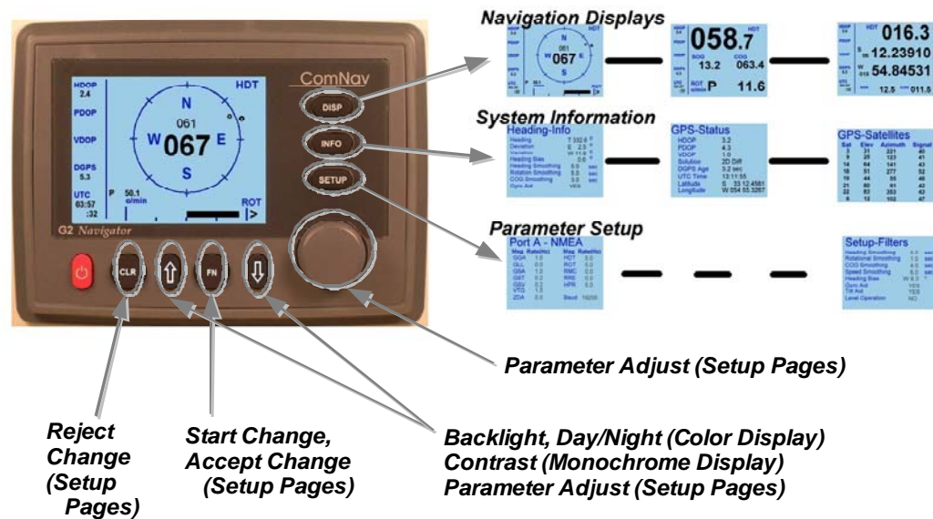
Figure 14 - Navigator G2 Display Head Displays and Buttons
