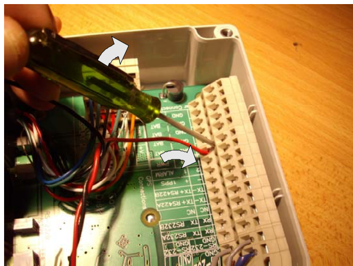
Figure 7 - Terminal Connection - Step 2
