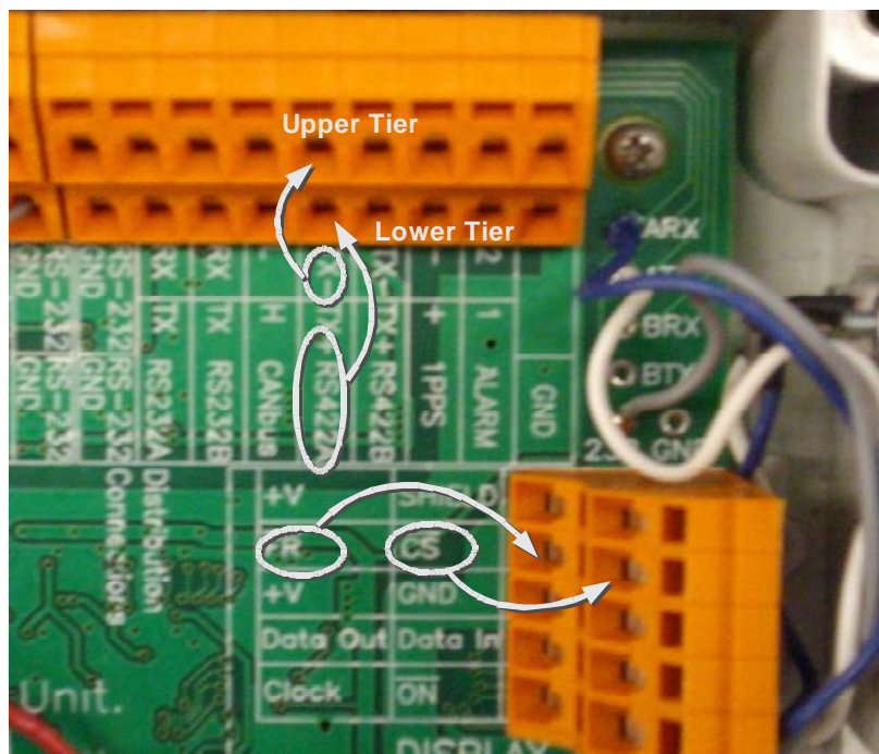
Figure 8 - Terminal Connection Silk Screen Labels
