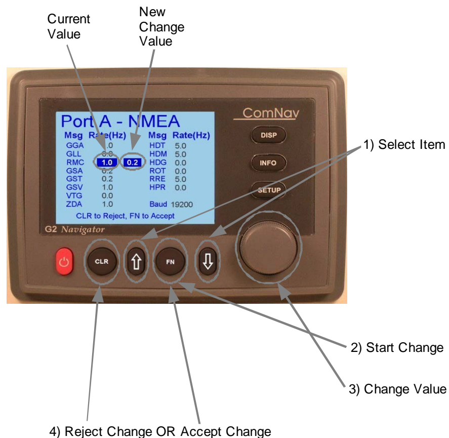
Figure 21 - Parameter Setup Page - Button Descriptions
