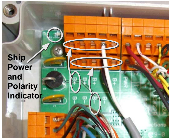
Figure 10 - Ship Power Connection
