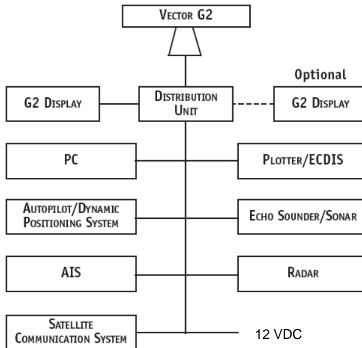
Figure 1 – Vector G2 System Connections
