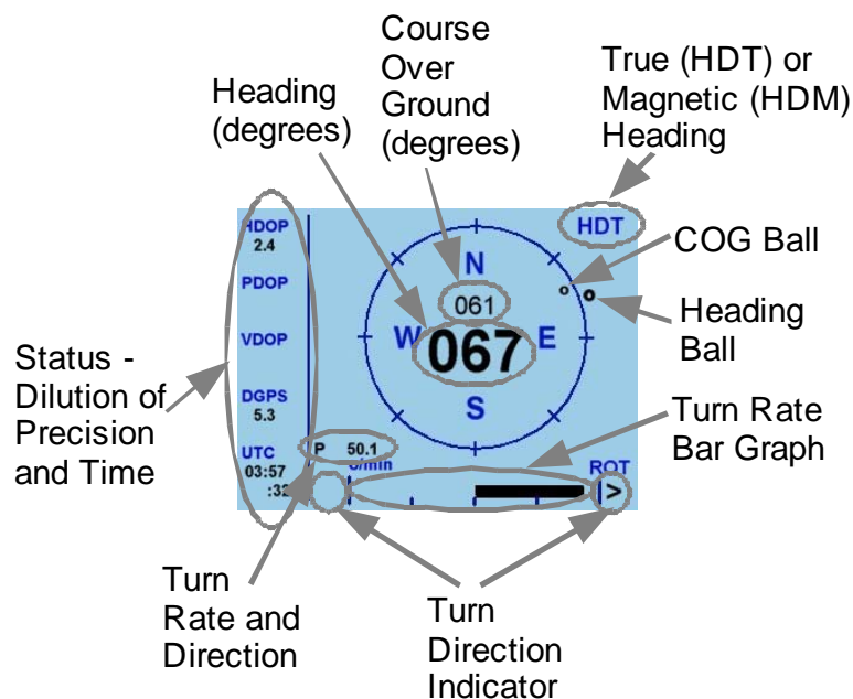
Figure 15 - Graphical Navigation Page Description
