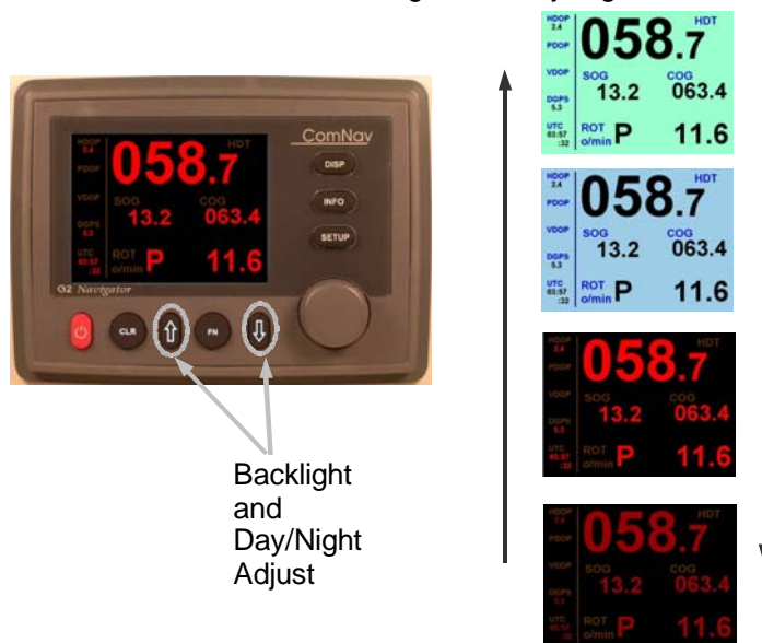
Figure 12 - Color Control Head Backlight and Day/Night Adjust
