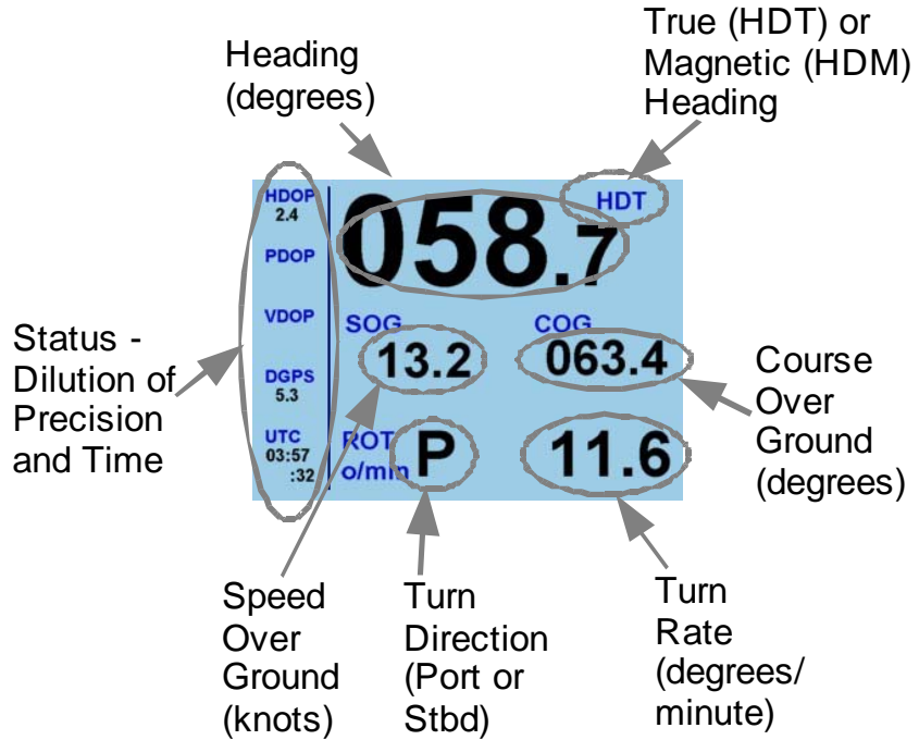
Figure 16 - Text Navigation Page Description
