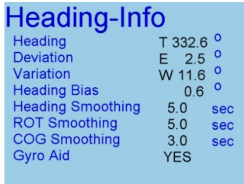
Figure 18 - Heading Information Page Description
