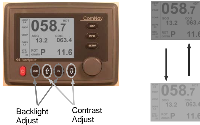
Figure 13 - Monochrome Display Head Contrast and Backlight Adjust
