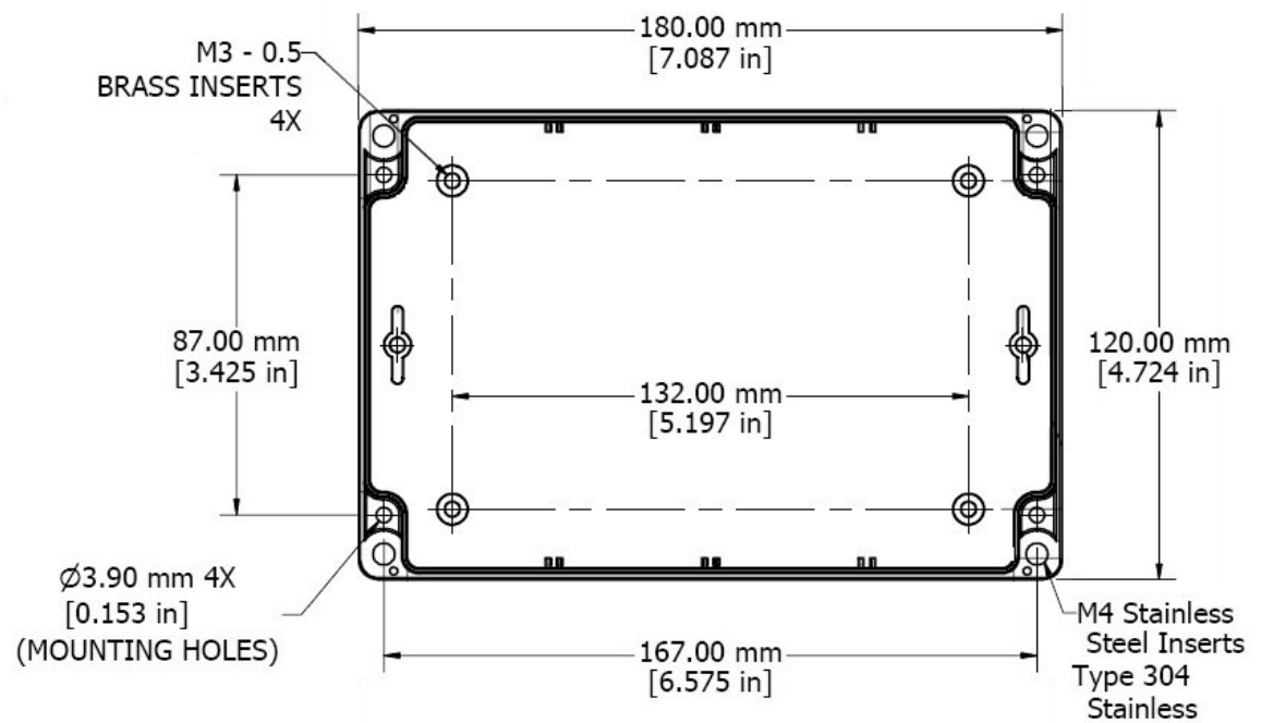
Figure 29 - Distribution Unit Dimensions
