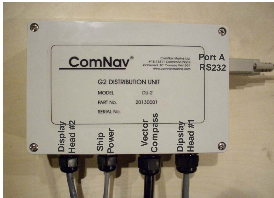
Figure 4 - Distribution Unit
