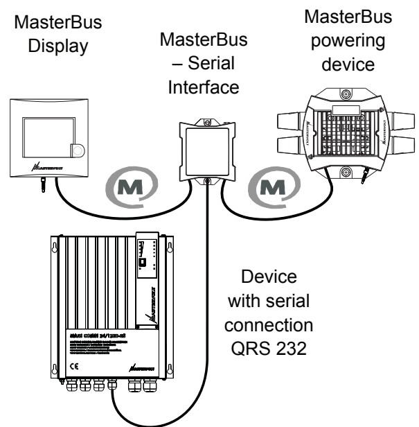
Figure 1: MasterBus-Serial interface in system
