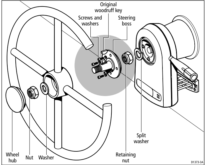
Fitting the SportPilot to 3/4 inch steering shaft
