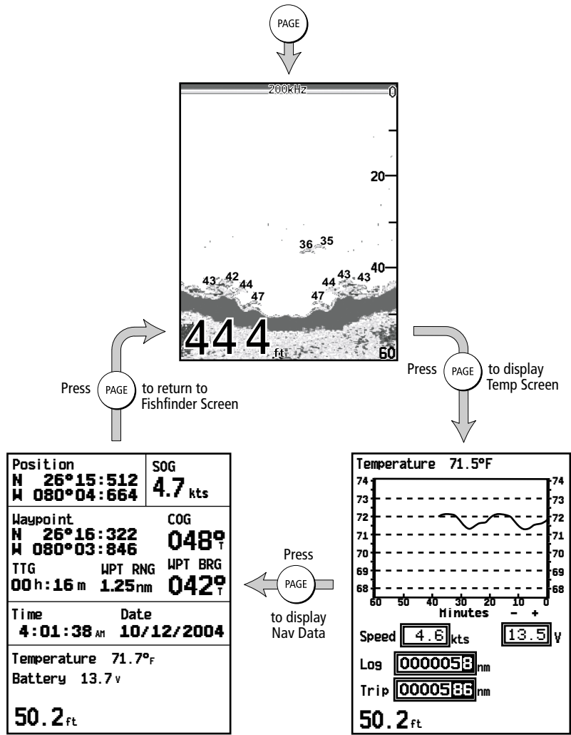
Figure 3-4: Display Pages
