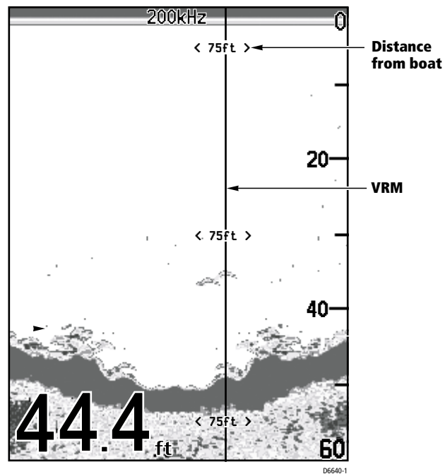
Figure 3-7: Using VRM
