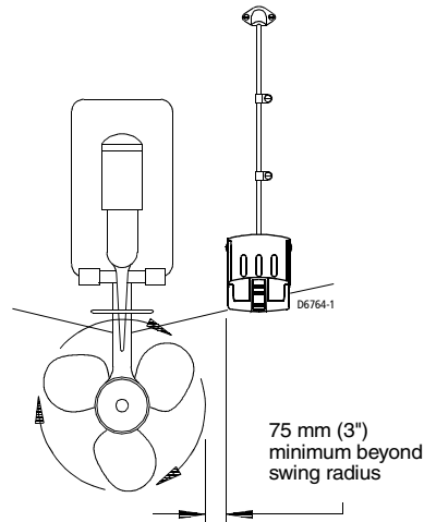
Figure 2-7: Mounting Location on Single Drive Boat
