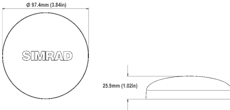
8.2 - AI50 GPS Antenna dimensions
