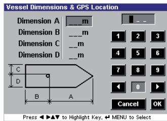
Fig. 4.12 – Vessel Dimensions & GPS Reference Entry Screen
