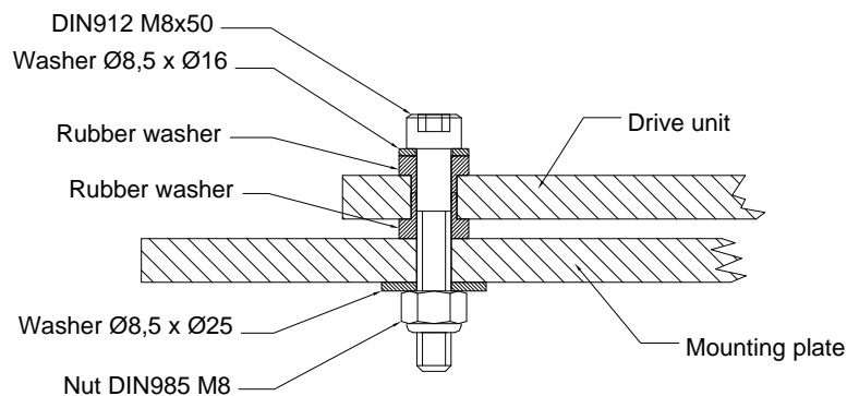
Figure 3-3 Reducing vibrations
