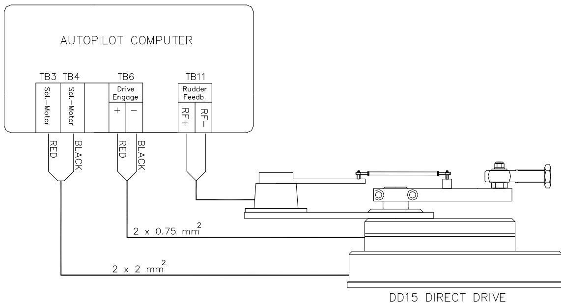
Figure 3-8 Autopilot connection
